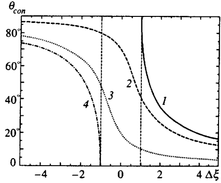
FIG. 2. Calculated dependence of the tilt angle \theta_{\text{con}} on the control surface on the anchoring parameter \Delta \xi at the different tilt angles \alpha_{\text{ref}} on the reference surface: 1— \alpha_{\text{ref}} = 90^\circ ; 2— \alpha_{\text{ref}} = 70^\circ ; 3— \alpha_{\text{ref}} = 20^\circ ; 4— \alpha_{\text{ref}} = 0^\circ .
