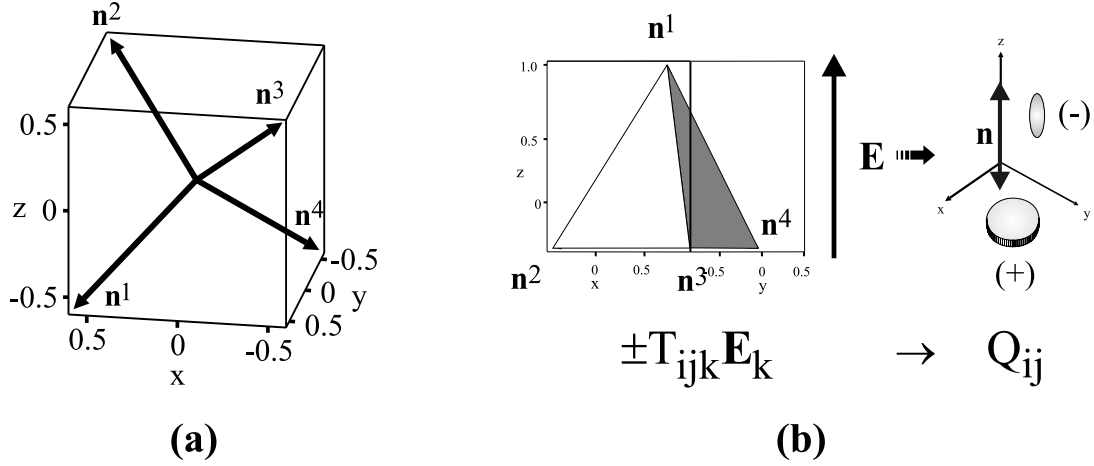
Fig. 1. The tetrahedric order parameter, T_{ijk} , lacks inversion symmetry. (a) is the Fel orientation [3] (b) T_{ijk} is oriented with \mathbf{n}^1 \parallel \hat{z} . Applying a field, \mathbf{E} \parallel \hat{z} , results in uniaxial orientational order \parallel \hat{z} [2].
