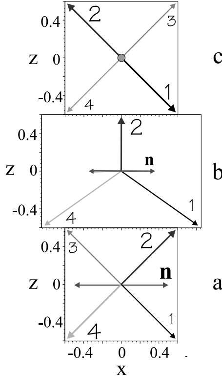
Fig. 2. A quarter pitch left-handed rotation for the isotropic tetrahedric (1, 2, 3 and 4 refer to the vectors in Fig. 1a) and a right-handed rotation of discs/rods for \mathbf{n} (2-headed arrow) shown in the \hat{x} - \hat{z} -plane ( \phi = 0 ). (a) qz = 0 : \mathbf{n} is in the \hat{x} - \hat{z} plane and \pm\pi/4 to the projections of the [2,3] and [1,4] tetrahedric 2-fold axes in this plane. (b) qz = \pi/4 : the [1, 4]-2-fold axis is in the \hat{x} - \hat{z} plane and the [2, 3] 2-fold axis is \perp to it. (c) qz = \pi/2 : \mathbf{n} is \perp \hat{x} - \hat{z} plane.
