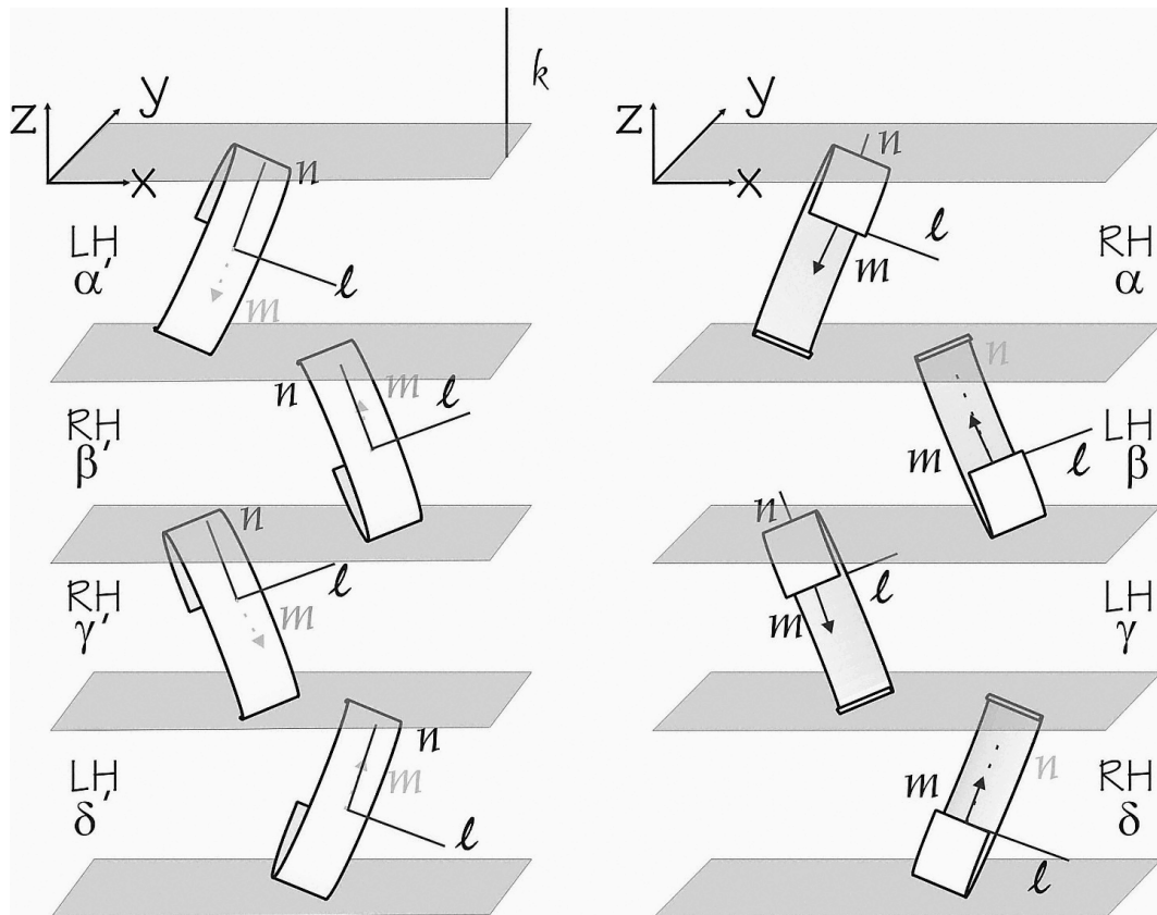
Fig. 2. Revised Fig. 2 of the right-handed ( \alpha, \delta, \beta', \gamma' ) and left-handed ( \beta, \gamma, \alpha', \delta' ) versions of smectic C_G .
