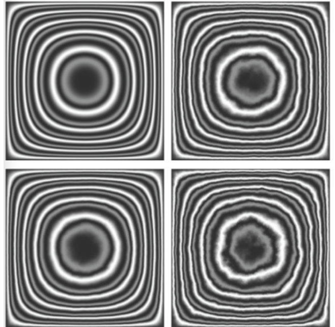
FIG. 2: The pattern at time 0.1 t_0 for a square cell (500 by 500 grid points) is shown as a function of the applied noise strength \xi_0 , which is 0 , 8\omega_L (left column), 16\omega_L , and 24\omega_L (right column). Note that \xi_0^2 \Delta^2 \Delta_t is the relevant parameter for noise, e.g., decreasing \Delta by some factor one must increase \xi_0 by the same factor for an equal noise effect, provided that \Delta is small compared to all other physical length scales (analogously for \Delta_t ).
