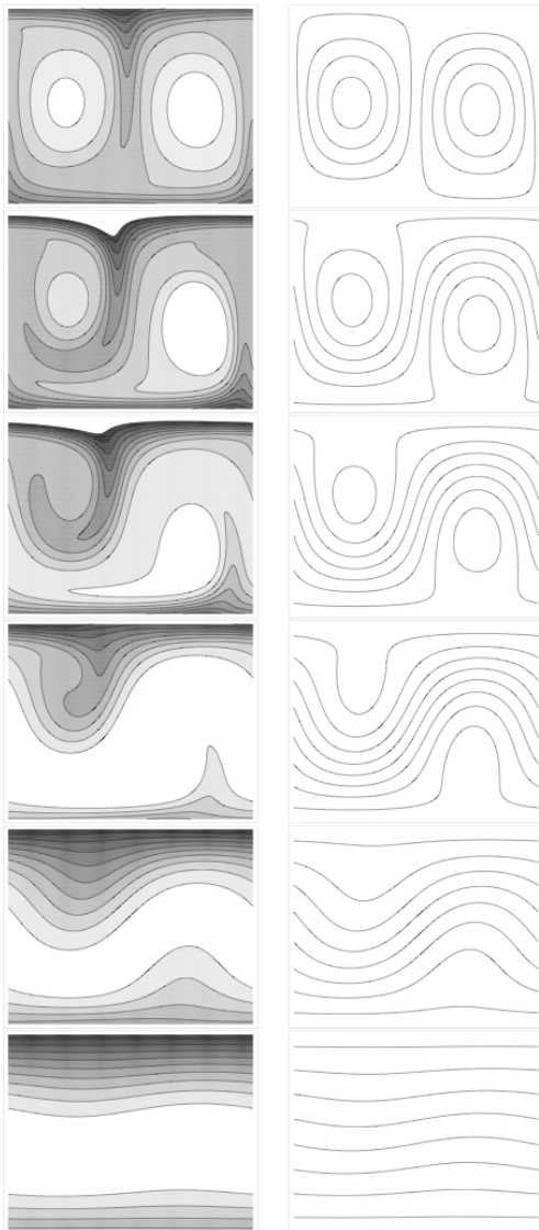
FIG. 13. Streamlines in the comoving frame (left) and the corresponding concentration field (right) for TWs at \sigma = 10 , L = 0.01 , \psi = -0.1 , k = 5 and A = 1 at frequencies \omega = 11, 9, 7, 5, 3, 1 (from top to bottom).
