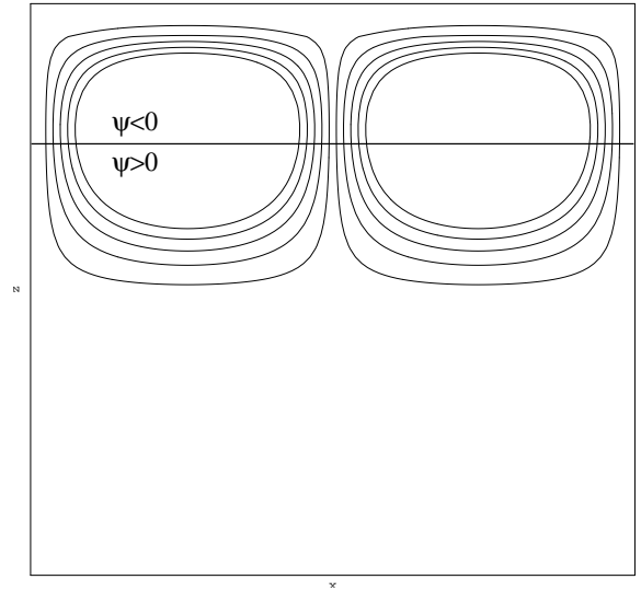
FIG. 4. The streamlines of the critical perturbation at L = 0.001 , \bar{\psi} = 0.25 , and A = 1 , the point denoted in Fig. 3.
