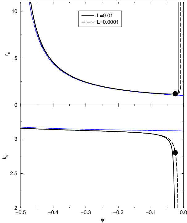
FIG. 5. (color online) The values (r_c, k_c) for heating from below and oscillatory convection as a function of \bar{\psi} for \sigma = 10 , two different L and A = 1 (thick black lines) compared to A = 0 (thin blue lines). The two dots denote the location of the structure in Fig. 6 in parameter space.
