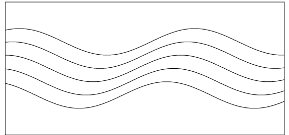
FIG. 12. A schematic picture of the streamlines in the comoving frame in the presence of a tilt in the convection rolls. The streamlines go from left to right.
