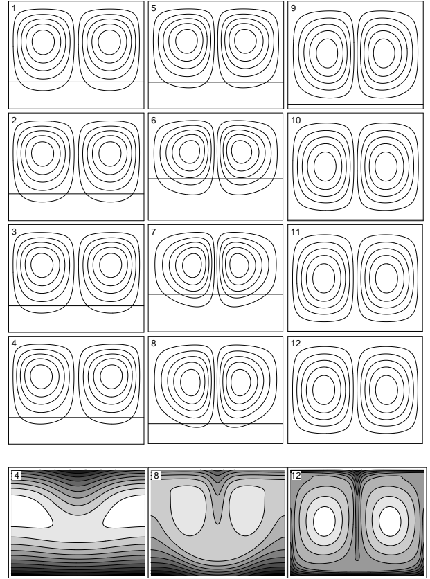
FIG. 9. Convection streamlines at the points denoted in Figs. 7 and 8. The horizontal line marks the lower end of the virtual cell. The last row shows selected concentration fields.
