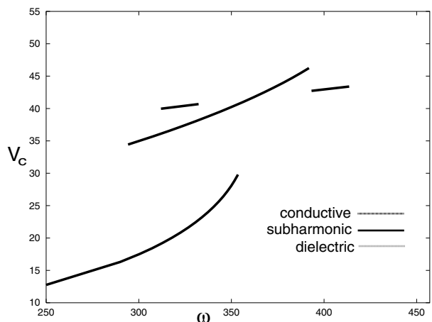
FIG. 9. Codimension-3 point: At the minimal value of the polarization ( p_0 = 4.5 for the parameters chosen), for which the subharmonic regime exists, the three different regimes have equal critical voltages at a certain external AC frequency \omega_3 \approx 361 . This is a codimension-3 point.
