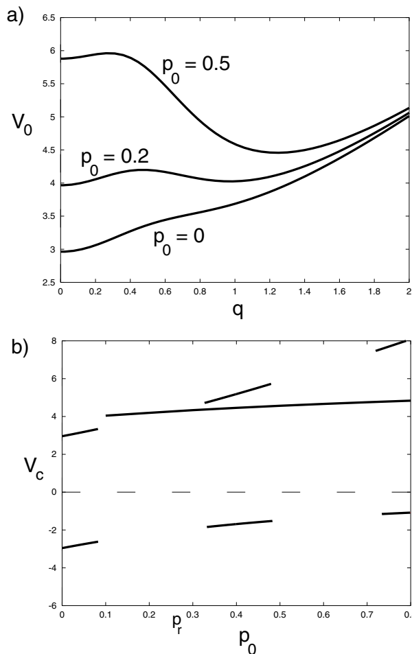
FIG. 2. a) The neutral curve for \epsilon_a = +0.6\epsilon_0 without polarization ( p_0 = 0 ) and with a polarization p_0 = 0.2 and p_0 = 0.5 parallel to the applied field ( V_0 > 0 ). In b) the threshold of electroconvection (solid lines) is compared with the that of the Frederiks transition (dotted lines) as a function of the polarization (for the positive value of \epsilon_a = 0.6\epsilon_0 ).
