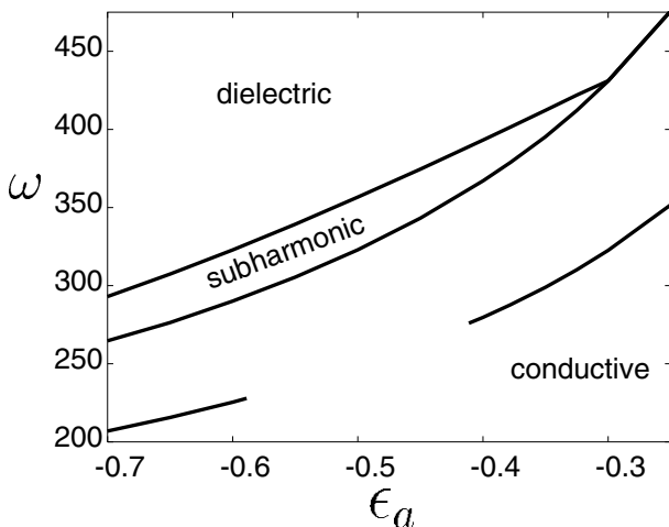
FIG. 10. The existence range of the subharmonic regime at various ac frequencies \omega as a function of the dielectric anisotropy for p_0 = 5 and \sigma_{\perp} = 133 fixed (both in dimensionless units cf. Eq.(28,29)) and \epsilon_{\perp} = 5.25 . The dashed line describes the codimension-2 line between the conductive and the dielectric regimes for p_0 = 0 .
