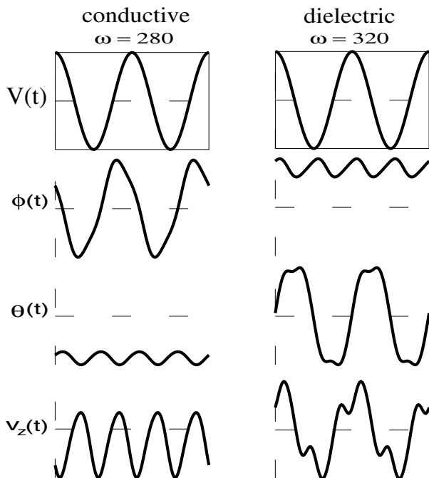
FIG. 4. The time dependence of the field variables is shown at the onset of electroconvection in the SmC phase (without macroscopic polarization). The temporal variations of the fields at the cell center ( z = 0 ) are plotted in arbitrary units for the conductive ( \omega = 280 ) and dielectric regime ( \omega = 320 ).
