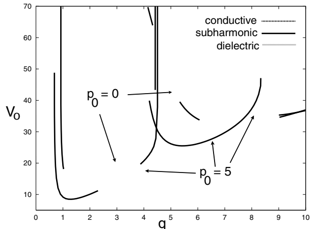
FIG. 5. Neutral curves V_0(q) are given for two different values of the polarization ( p_0 = 0 and 5) at the frequency \omega = 180 of the applied voltage. The upper (lower) curve in the conduction regime (dashed lines) and the lower (higher) one in the dielectric regime (dotted lines) are calculated for p_0 = 0 ( p_0 = 5 ). For finite polarizations the additional subharmonic regime occurs at intermediate q values (solid line).
