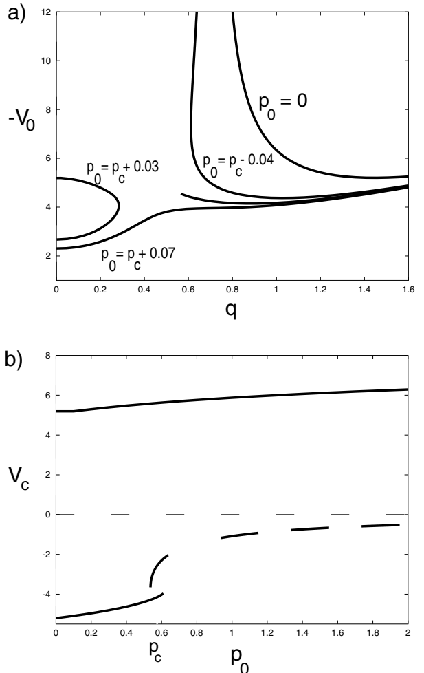
FIG. 3. The neutral curve (a) and the comparison of convective and Frederiks instabilities (b) just like in Fig.2 but for negative dielectric anisotropy \epsilon_a = -0.38\epsilon_0 , where p_c = 0.54 .
