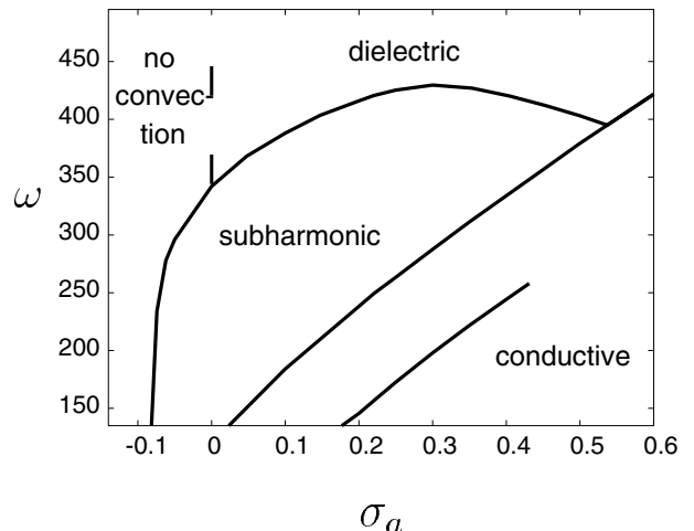
FIG. 11. The solid lines indicate the existence ranges of the different instability regimes at various ac frequencies as a function of the conduction anisotropy \sigma_a for p_0 = 5 and \sigma_{\perp} = 133 and \epsilon_{\perp} = 5.25 ; \epsilon_a = -0.38 . The dashed line describes the codimension-2 line between the conductive and the dielectric regimes for p_0 = 0 .
