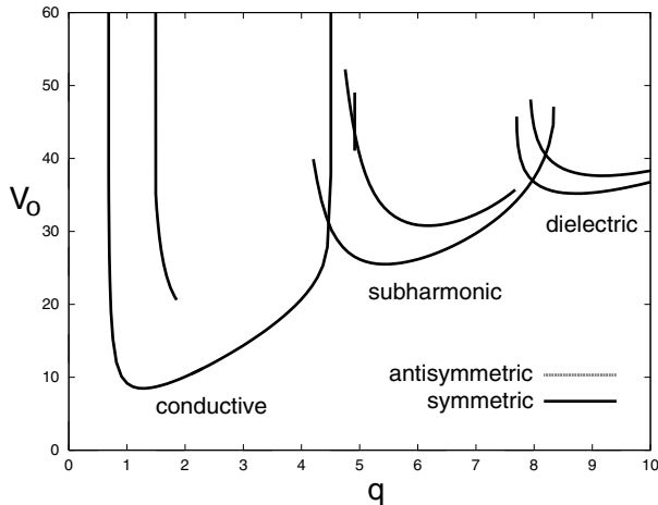
FIG. 6. Three different instability regimes: (a) The conductive, (b) the subharmonic and (c) the dielectric regime. The solid lines show the neutral curves V_0(q) for branches symmetric under z -reflection, Eq.(41), while the dash-dotted lines belong to antisymmetric solutions. Here the parameters (applied AC frequency \omega = 180 and spontaneous polarization p_0 = 5 ) are chosen such that the lowest minimum of the neutral curves belongs to the conductive regime.
