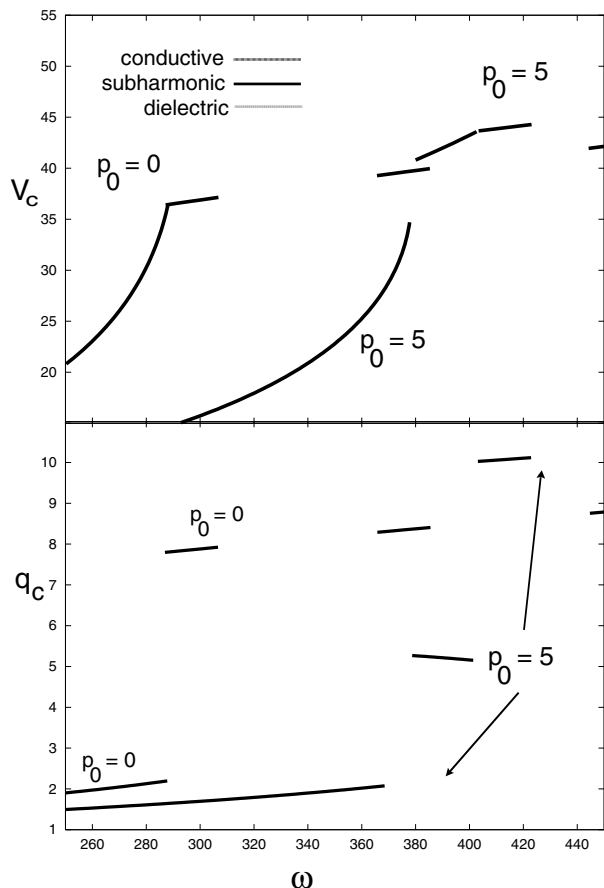
FIG. 8. Onset of instability: a) The critical voltages V_c = V(q_c) , b) the critical wavenumbers q_c , of the three regimes as a function of the applied AC frequency. For low or vanishing polarization p_0 there are only two regimes, while for p_0 > 4.5 (for the parameters chosen) there is in addition the subharmonic regime at intermediate frequencies. At those frequencies, where the instability switches from one regime to the other, the critical wavevector shows a jump.
