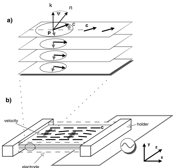
FIG. 1. a) A stack of SmC* layers is shown, for which the orientation of the director \mathbf{n} changes from layer to layer gradually. b) Similarly to experiments with SmA films [17] we suggest the sketched experimental setup for the study of electroconvection in SmC*-films. A rectangular freely suspended SmC*-film is plotted with the electrodes parallel to x -direction. The length of the film is assumed to be much longer ( \parallel x ) than wide ( \parallel z ).
